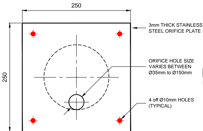
STAINLESS STEEL ORIFICE PLATE DETAIL SCALE 1:5
