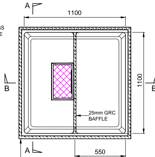
OPEN TANK PLAN VIEW SCALE 1:25
