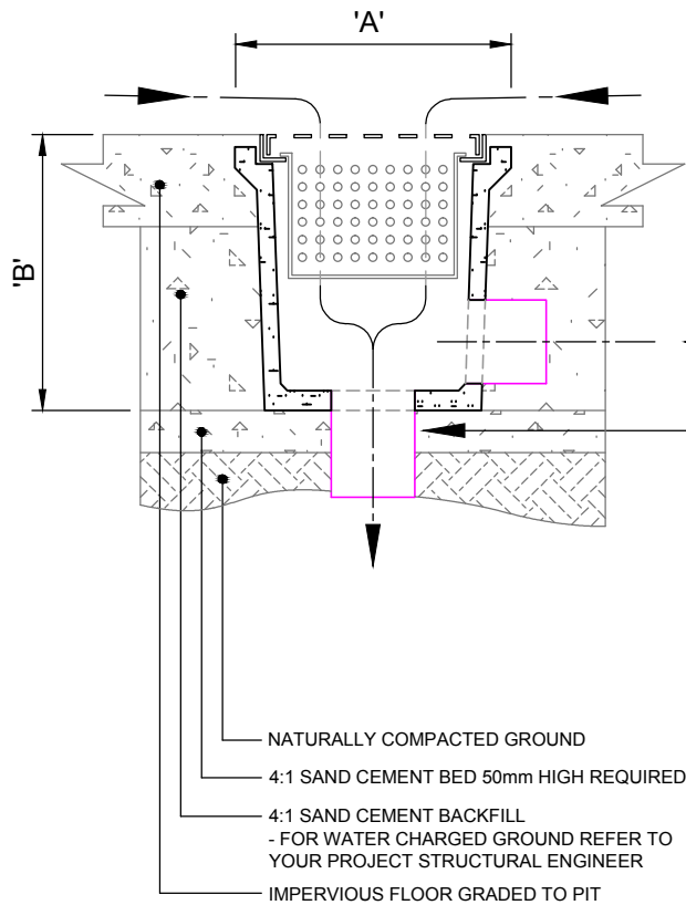
SIDE SECTION SCALE 1:10
