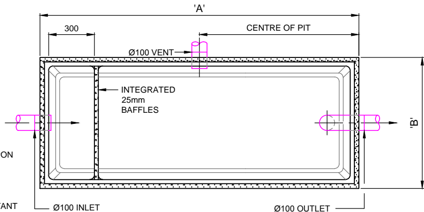
OPEN TANK PLAN VIEW SCALE 1:25
