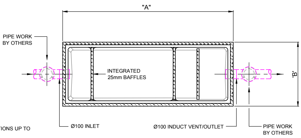
OPEN TANK PLAN VIEW SCALE 1:25
