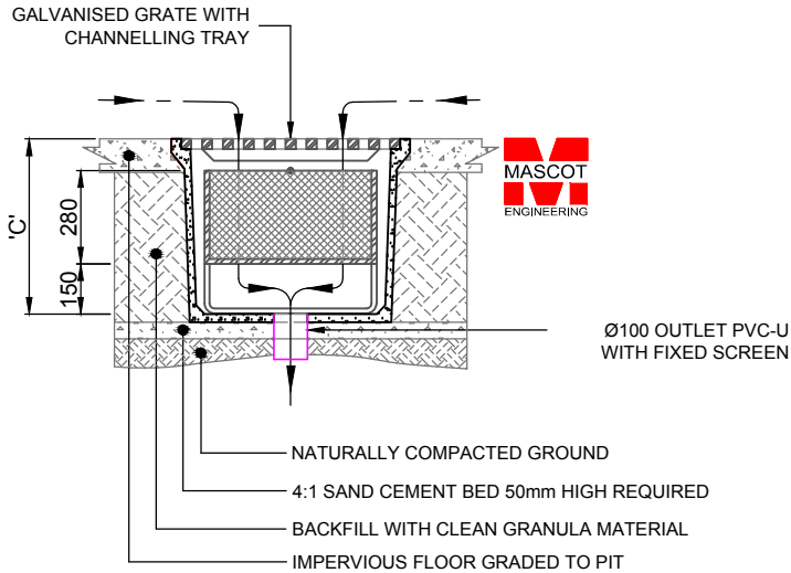
SIDE SECTION SCALE 1:25
