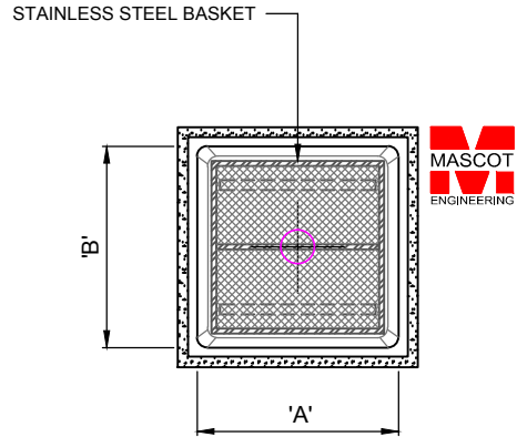
OPEN TANK PLAN VIEW SCALE 1:25
