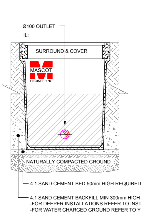
END SECTION SCALE 1:25
