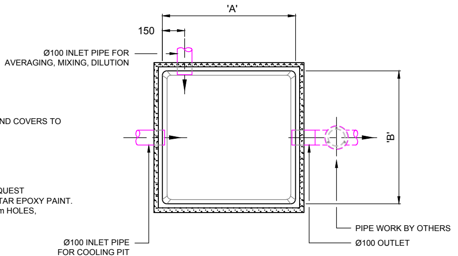
OPEN TANK PLAN VIEW SCALE 1:25
