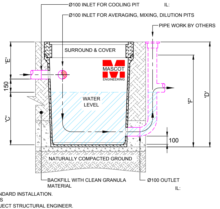
SIDE SECTION SCALE 1:25
